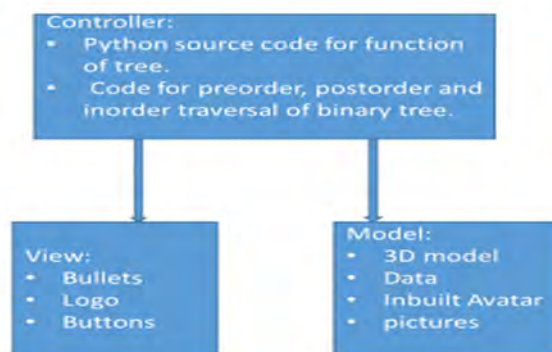
Fig. 3. Shows the MVC architecture used in the GTI module.
